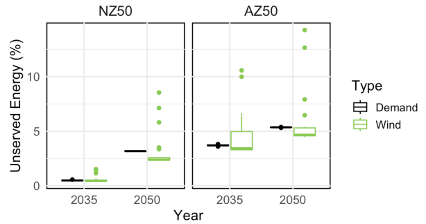
Figure 1: Boxplot of unserved energy (%) from a probabilistic analysis of load and wind (Monte Carlo analysis)
