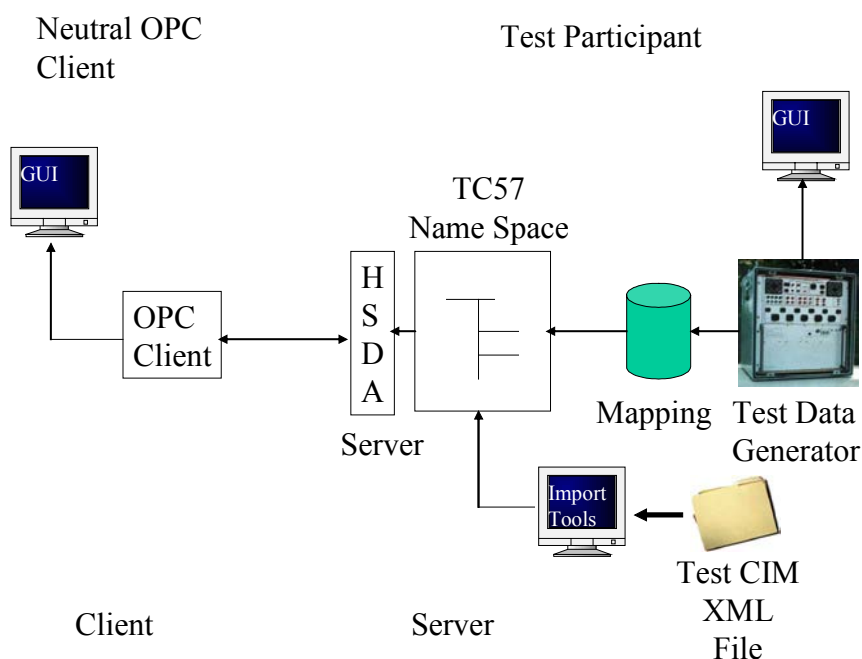
Figure 2-1 Test Set-up for HSDA Conformance Testing
