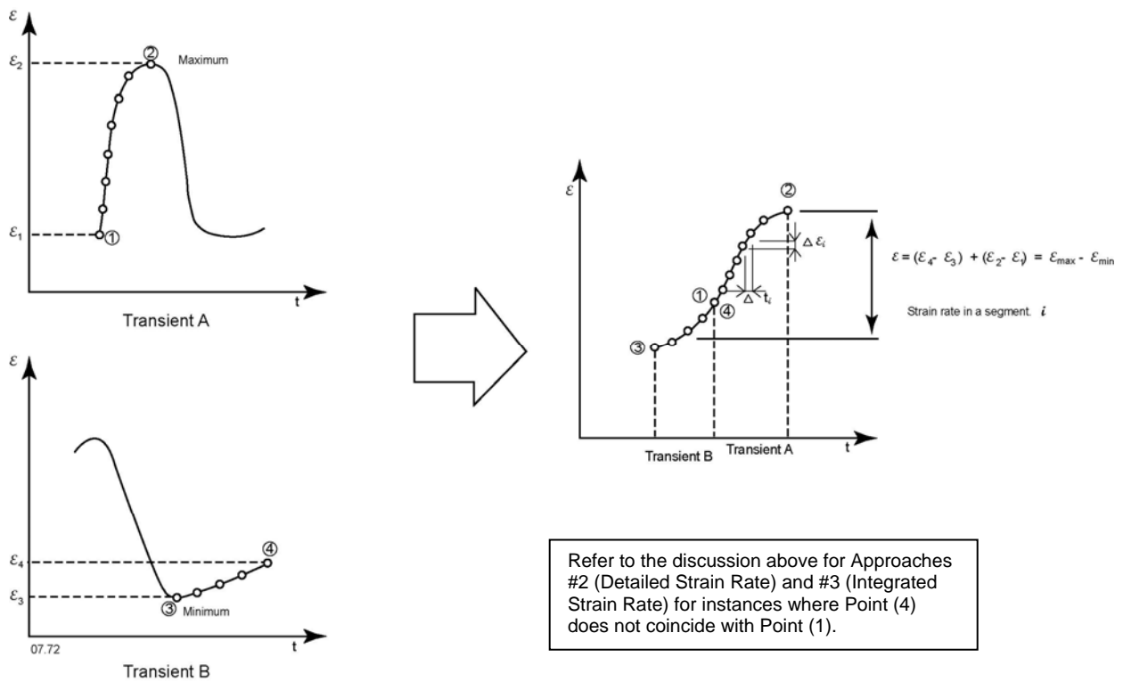
Figure 4-5 Detailed and Integrated Strain Rate Calculation
