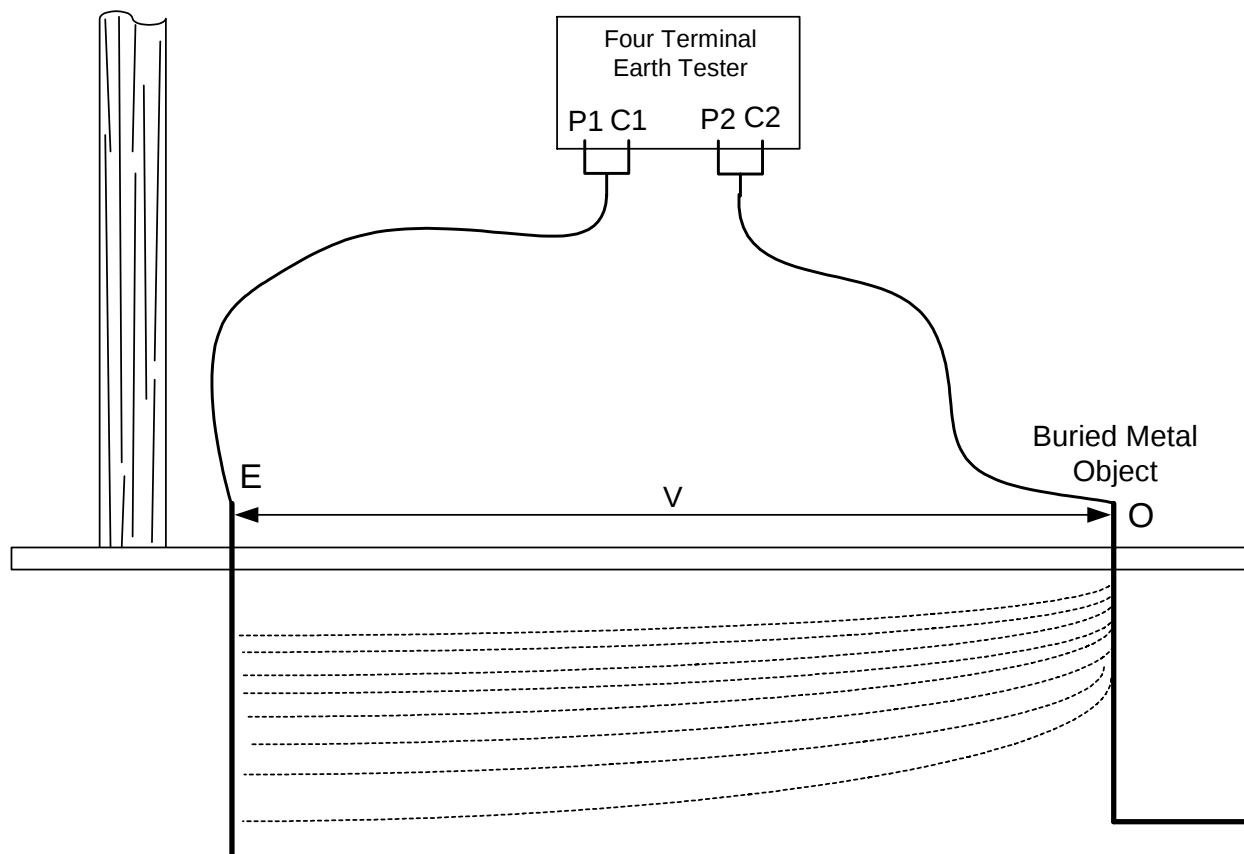
Figure 3-5 Two Point Test Method
