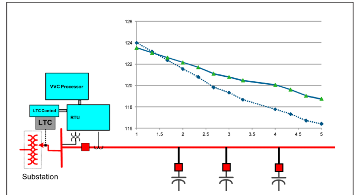
Figure 7(b): Capacitor Switching
