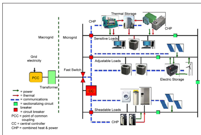
Figure 4: Microgrid Configuration
