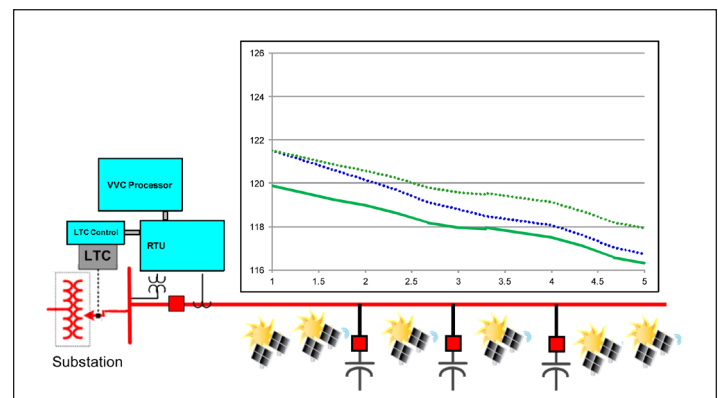
Figure 7(e): Final voltage reduction
