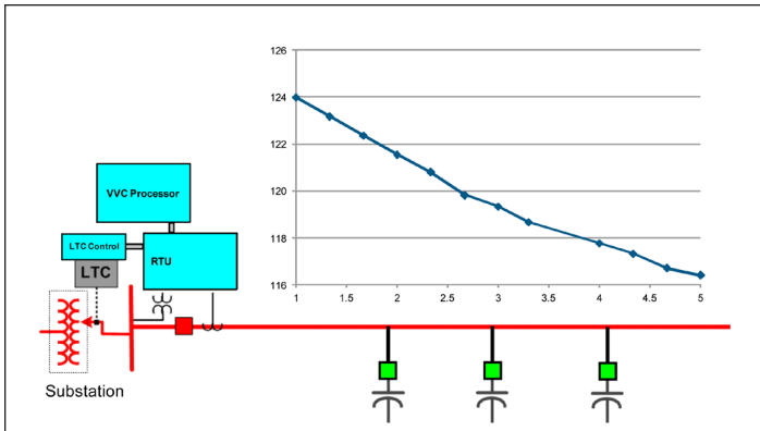
Figure 7(a): Original voltage profile
