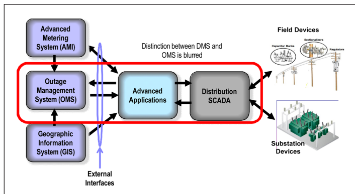
Figure 1: Integrated DMS Concept
