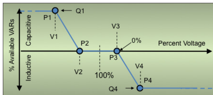
Figure 6: Volt-Var Curve Configuration via Array of Points
