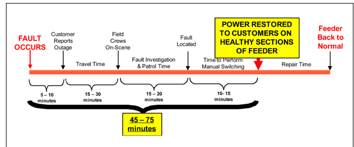
Figure 3: Time Line for Service Restoration (without FLISR)
