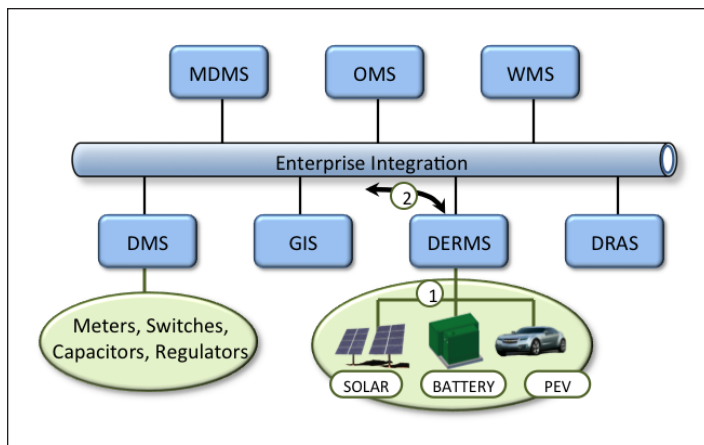
Figure 5: Utility Enterprise Diagram
