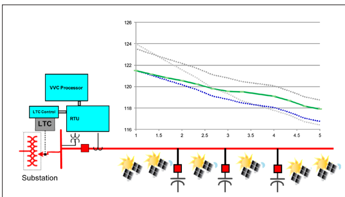
Figure 7(d): Smart inverter Impact on voltage
