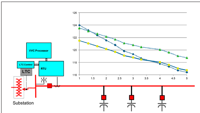
Figure 7(c): Volt regulator Operation
