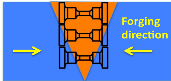
Figure 3-6 Orientation of tensile specimens cut from weldments
