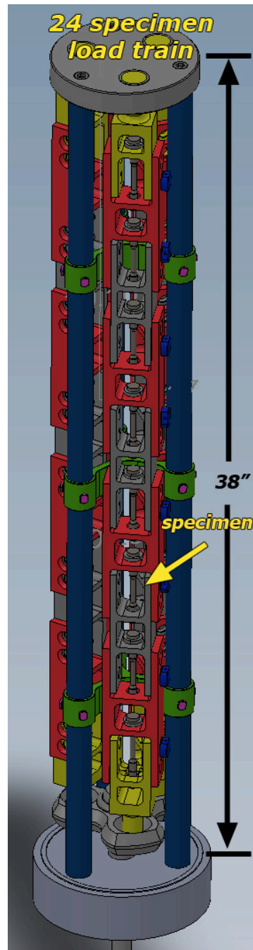
Figure 4-1 Early 3-string design showing a 24-specimen load train
