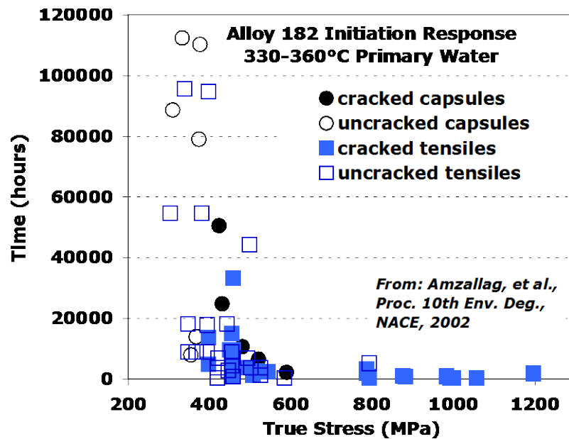
Figure 6-1 Alloy 182 SCC initiation test results by Amzallag, et al. [6]
