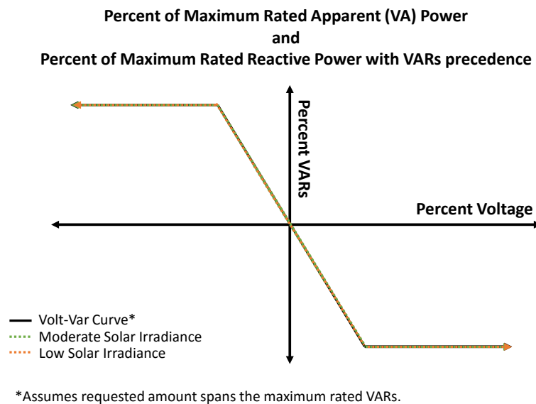
Figure 11-2 Example of both percent of maximum rated apparent (VA) power and percent of maximum rated reactive power with VARs precedence
