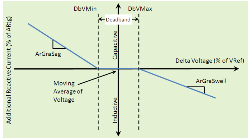
Figure 18-1 Dynamic reactive current support function, basic concept
