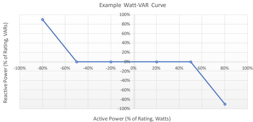
Figure 24-2 Example watt-VAR array where the curve does not extend the full width of the inverter’s active power operating range
