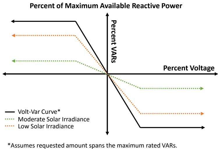
Figure 11-4 Example of percent of maximum available reactive power, with watt precedence
