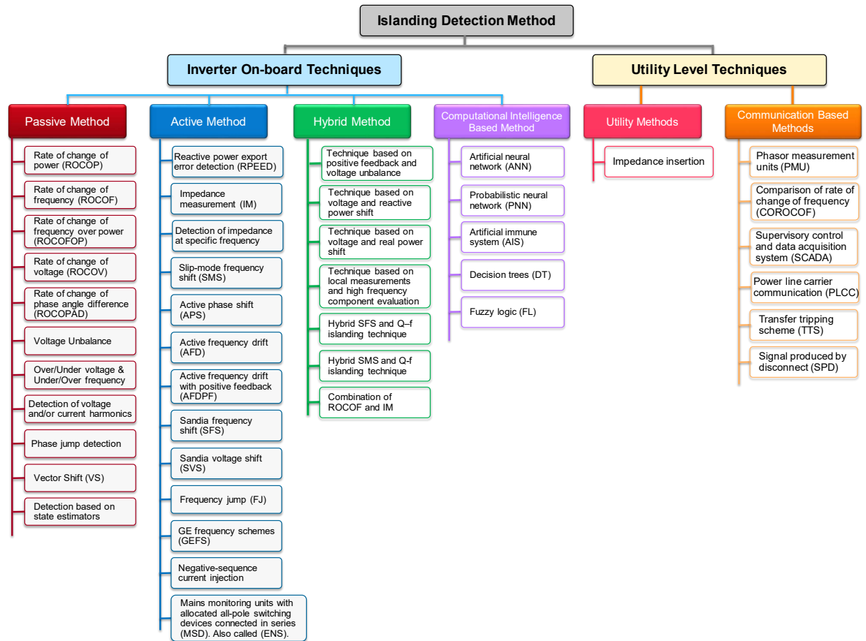
Figure 2-1 Classification of islanding detection methods
