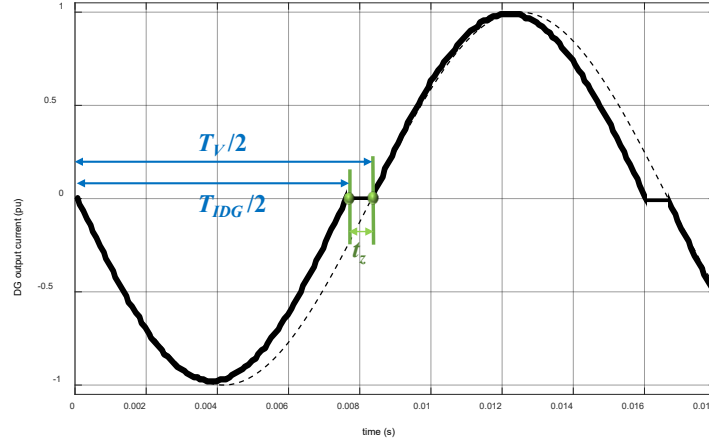
Figure 2-3 DG output current using AFD.
