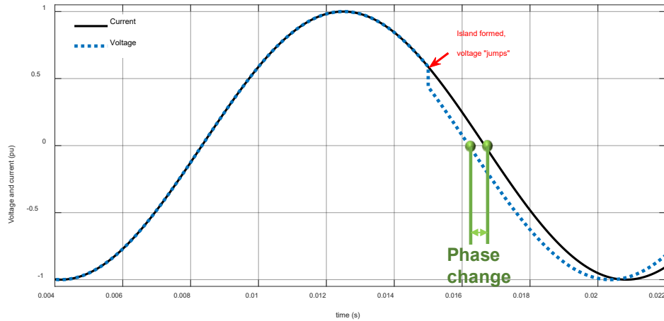
Figure 2-2 Phase jump islanding detection.
