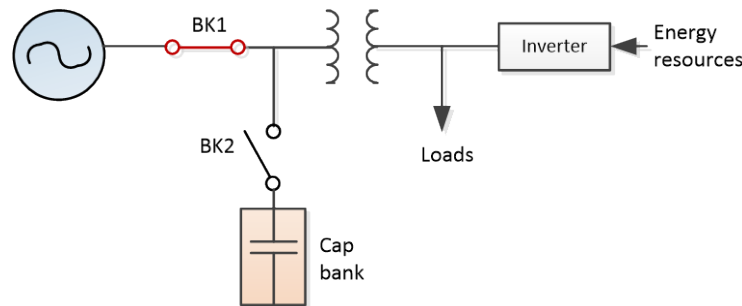
Figure 2-4 Impedance insertion based islanding detection.
