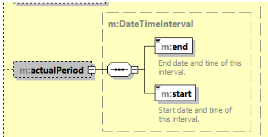
Figure 2-1 Schema view of “actualPeriod” data type
