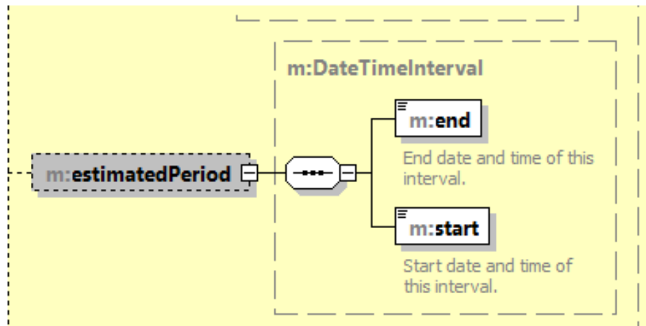
Figure 2-2 Schema view of “estimatedPeriod” data type
