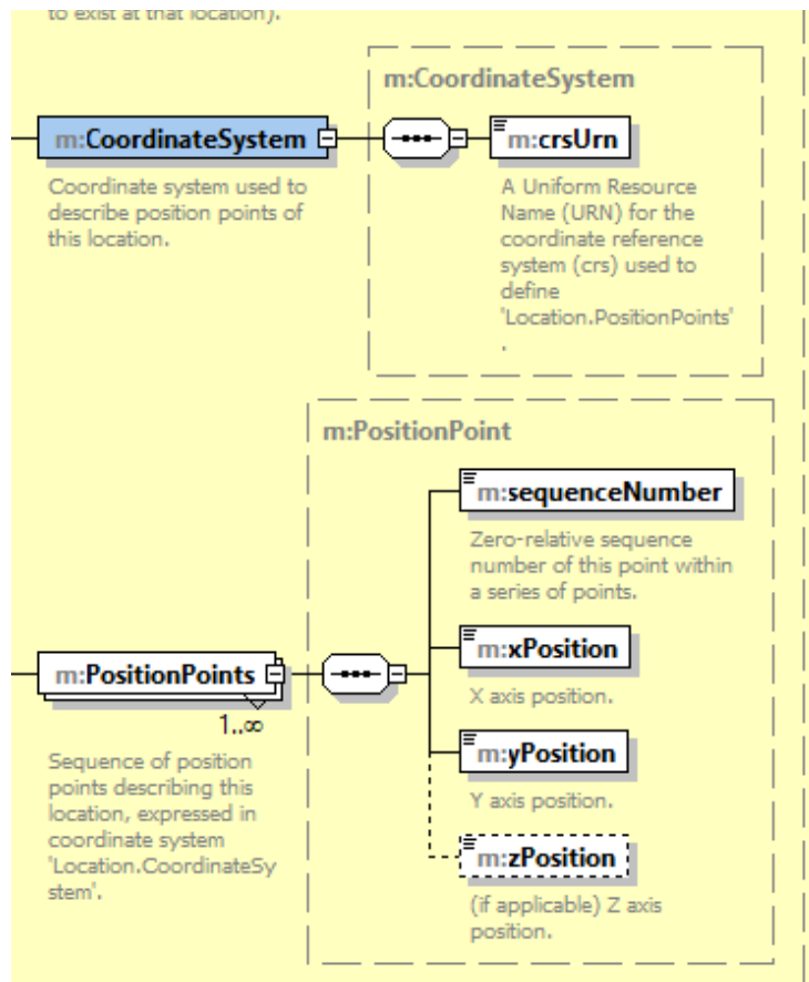
Figure 2-6 Schema view of “CoordinateSystem” and “PositionPoints” data types
