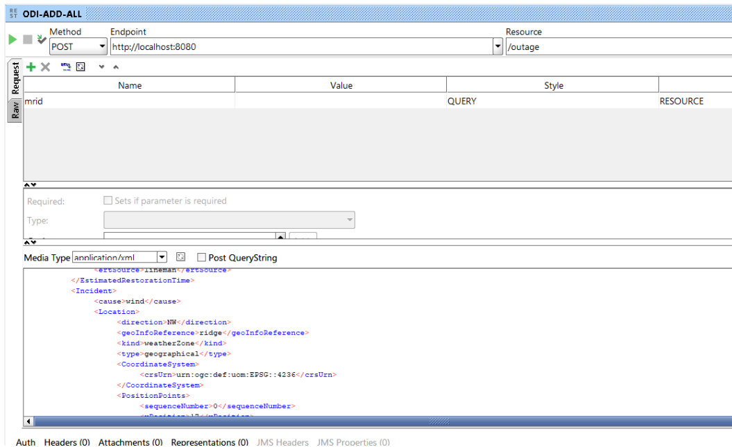
Figure 1-3 Sending a POST message in SoapUI using their REST interface
