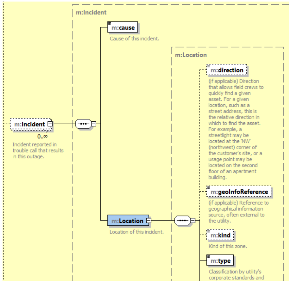
Figure 2-4 Schema view of "Incident" data type
