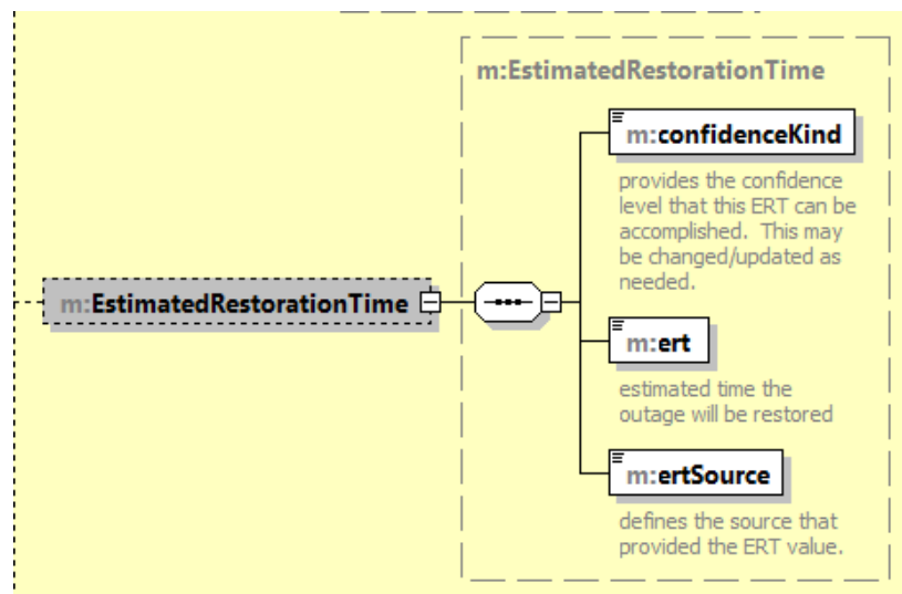
Figure 2-3 Schema view of “estimatedRestorationTime” data type
