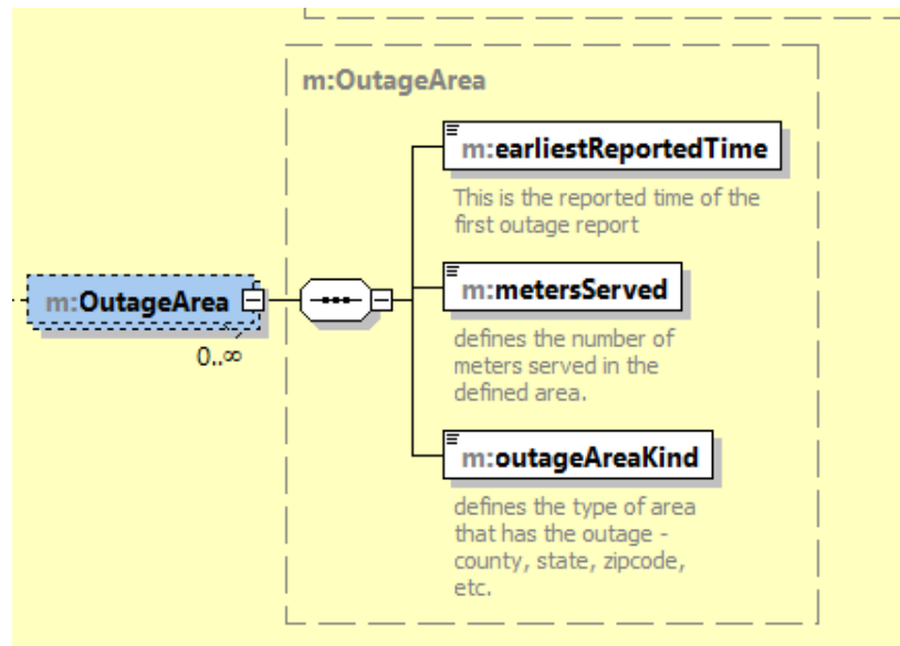
Figure 2-7 Schema view of “OutageArea” data type
