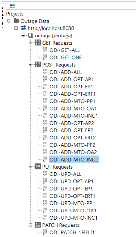
Figure 1-2 Same file structure for this test script in SoapUI
