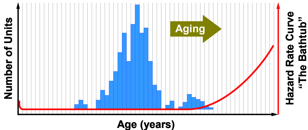
Figure 4-2 A Hypothetical Equipment Age Distribution and Failure Rate Curve
