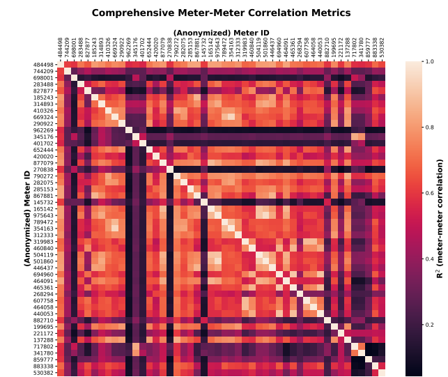
Sample results from the methods used for inferring smart meter organization within a small substation: (top) heat map visualizing statistical similarity between all pairs of meters based on 1 full year of power, voltage, and current time-series data; and (right) hierarchical clustering results using similarity values (meter identification colors correspond to Ameren’s internal grouping label)
