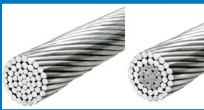
Figure 1. Conventional AAAC, ACAR and ACSR Conductors
