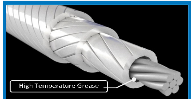
Figure 2. Gap-Type Conductor [Courtesy of Lamifil]
