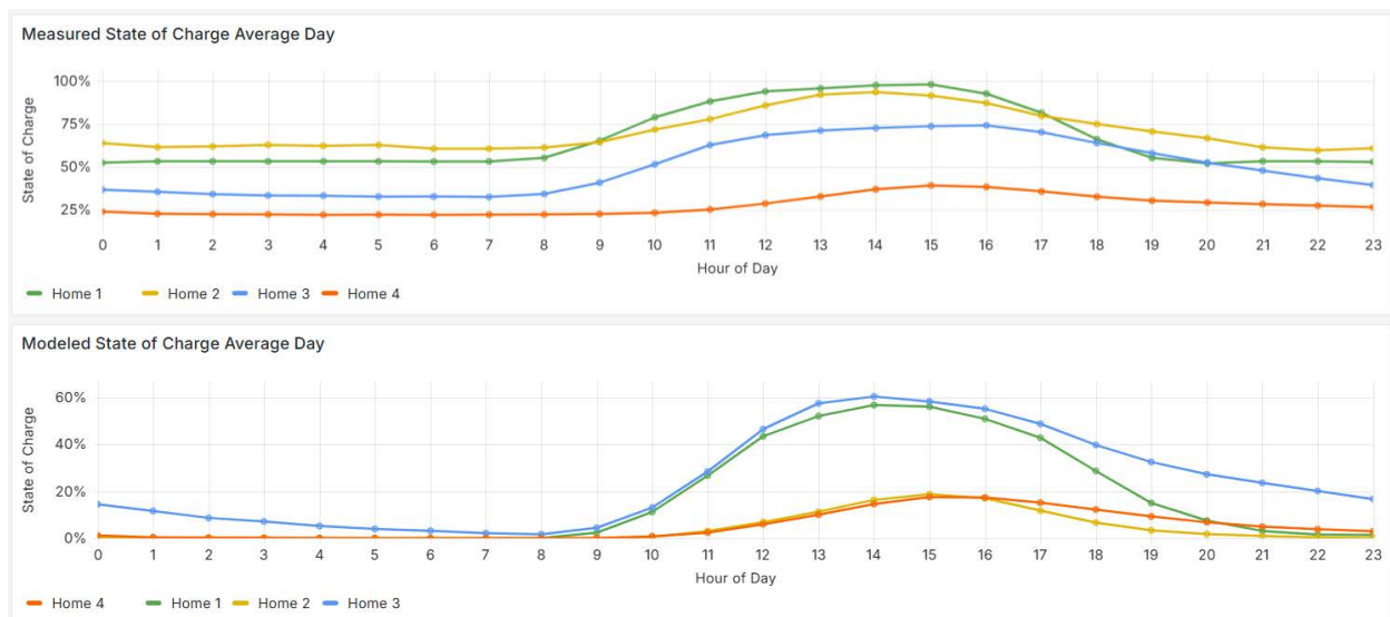
Figure 7. State of charge timeseries for the homes on the average day.
