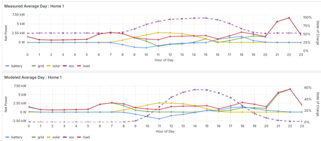
Figure 9. Average day of loads, generation, and dispatch for Home 1 in December, depicting EV charging patterns.
