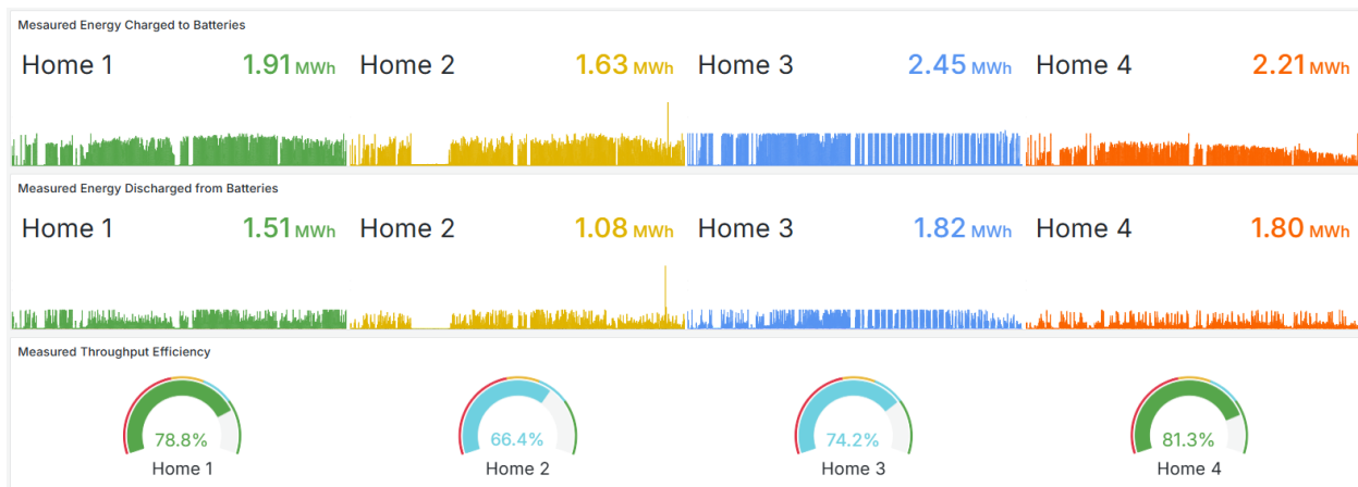
Figure 4. Throughput energy and efficiency for the homes measured operation.
