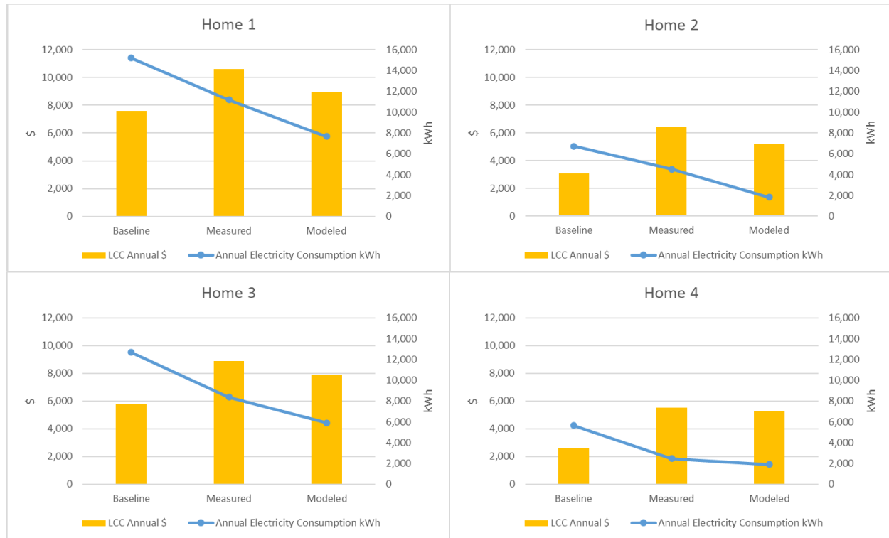
Figure 3. Annual LCC and annual electricity consumption of each home.
