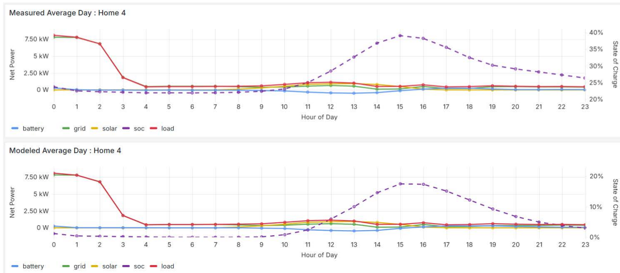
Figure 10. Average day of loads, generation, and dispatch for Home 4 in December, depicting EV charging patterns.
