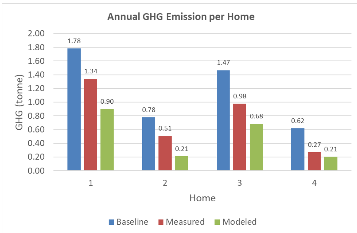
Figure 1. Annual GHG emissions across baseline, measured, and modeled scenarios.
