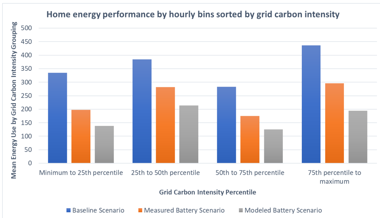
Figure 2. Mean power draw grouped by grid carbon intensity.
