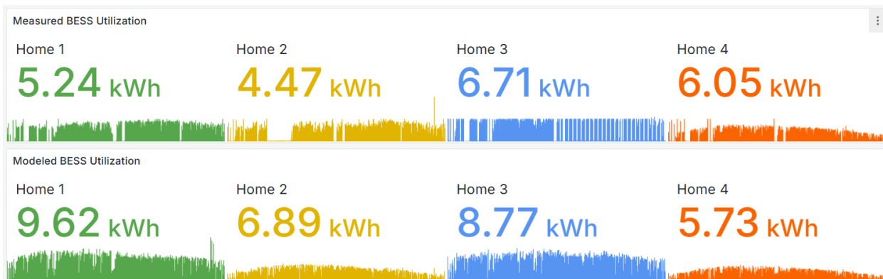
Figure 8. Measured vs. modeled BESS utilization over the analysis year.
