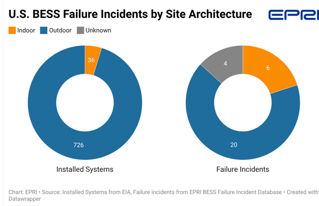
Figure 16. Comparison of Failure Incident Count by Architecture, U.S. Only
